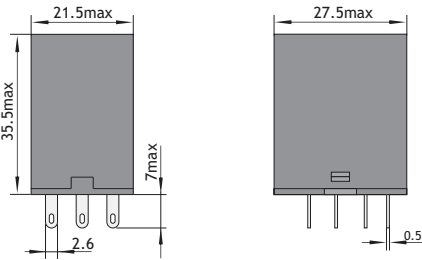
JZX-22F(D)/3-05
